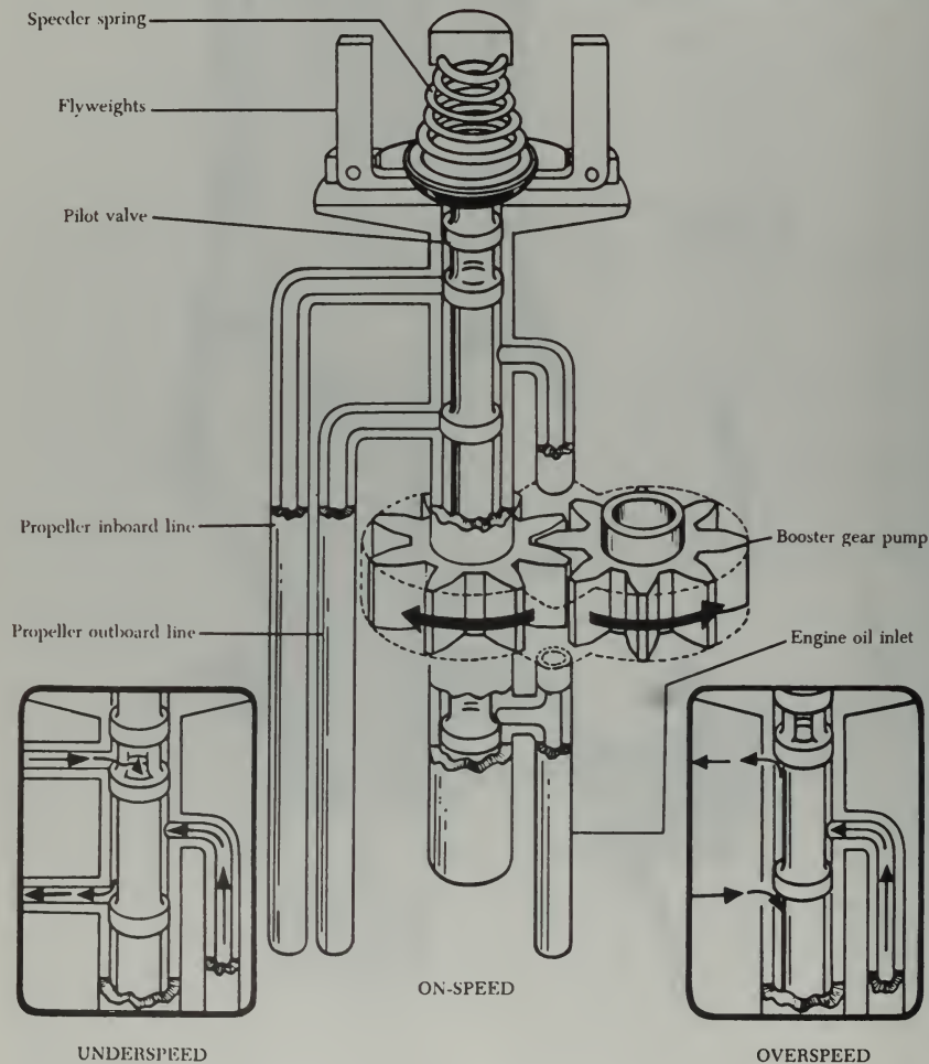
FIGURE 7-23. Propeller governor operating diagram.
